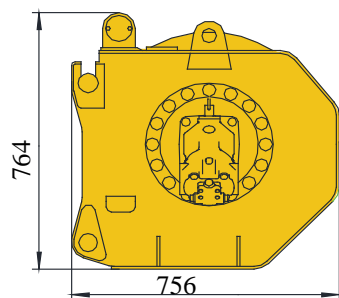
副起升机构(含钢丝绳) 1060kg Auxiliary winch (wire rope included) 1060kg
